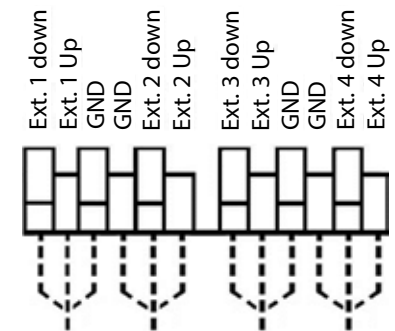
Fig.: Connection external push buttons
